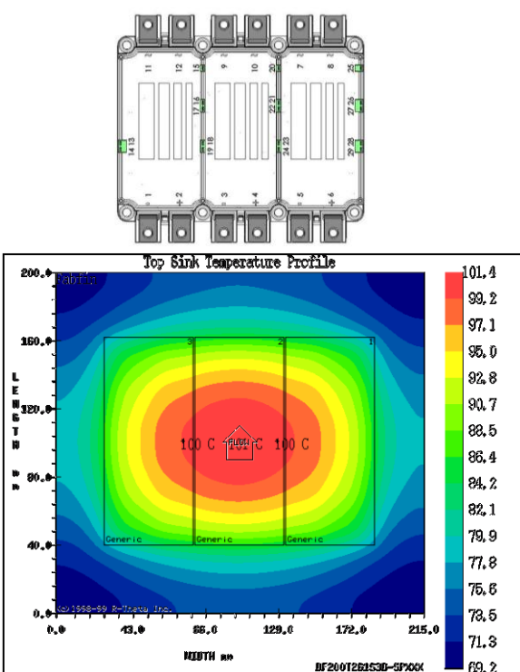
Fig. 8-11 SEMiX "33c" six-pack module
