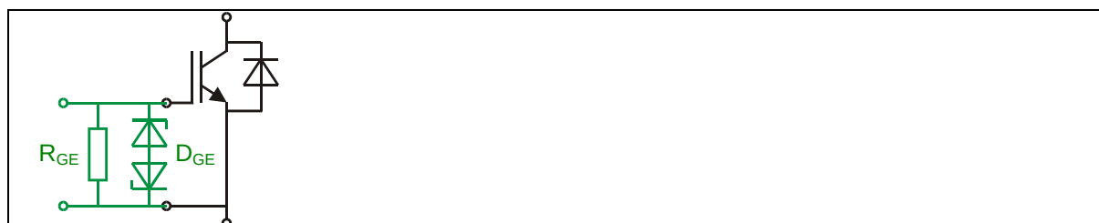
Fig. 8-5 Gate clamping circuit
