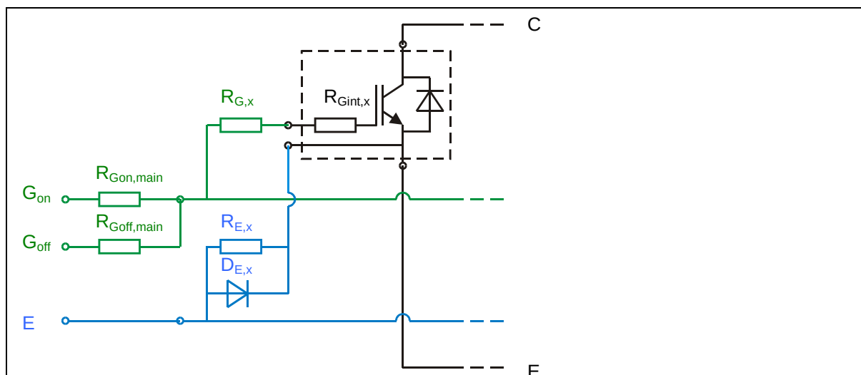
Fig. 8-4 How to understand the value for R_{G,int} given in the data sheets
