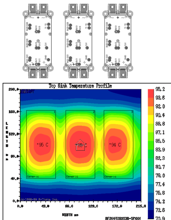
Fig. 8-12 3 x SEMiX "3" module for optimised thermal management
