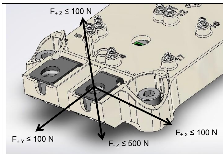
Fig. 9-5 Maximum forces at the main terminals
