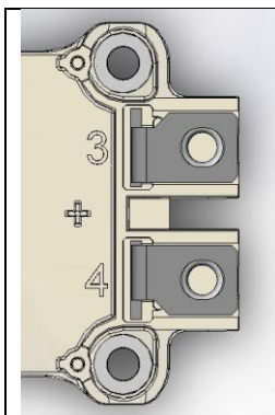
Fig. 9-6 Detail: AC terminal of SEMiX
