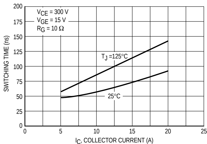
Figure 15. Inverter Switching Time t_r versus Collector Current I_C
