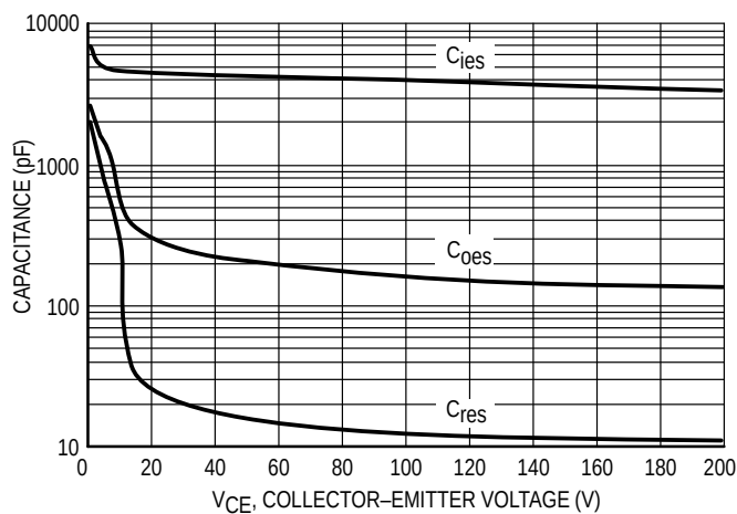
Figure 17. Output Inverter Capacitance versus Collector Voltage V_{CE}
