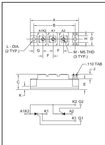
CM430890 Dual SCR POW-R-BLOK™ Modules 90 Amperes/800 Volts
