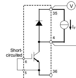
Brake IGBT
