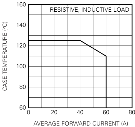
ALLOWABLE CASE TEMPERATURE VS. AVERAGE FORWARD CURRENT
