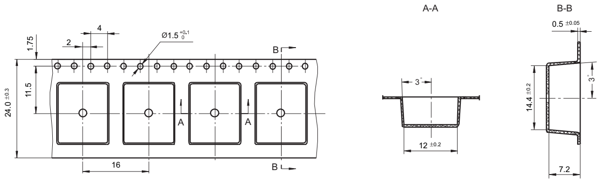
Tape Dimensions
