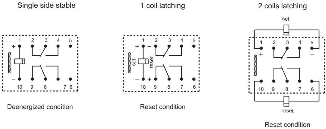
Wiring Diagram (Bottom view)
