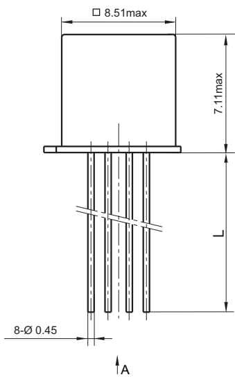
Outline Dimension
