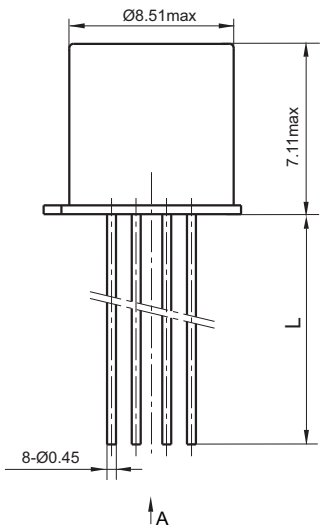
Outline Dimension
