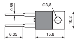
TO-220A (TO-220AC)
