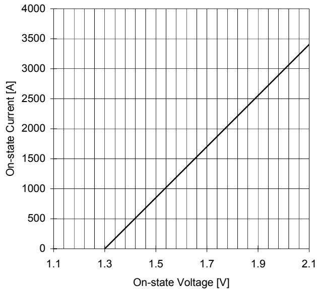
ON-STATE CHARACTERISTIC T_J = 120\text{ }^\circ\text{C}
