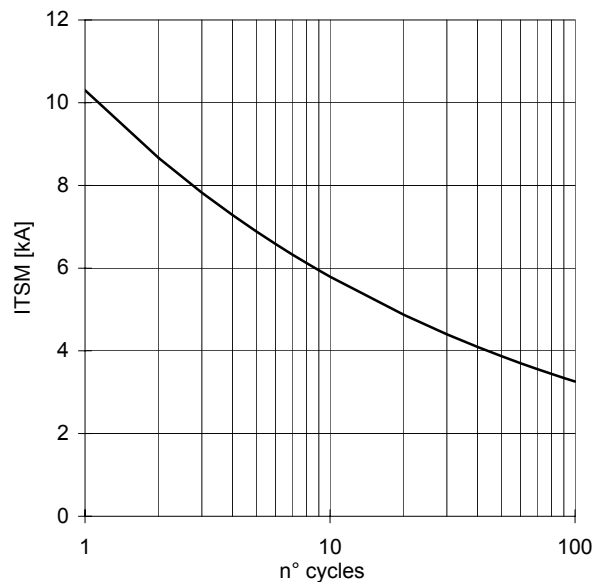
SURGE CHARACTERISTIC T_J = 150^\circ\text{C}
