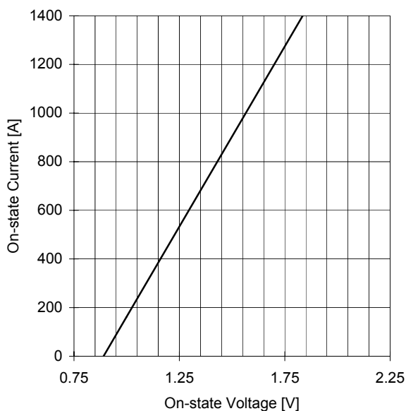
ON-STATE CHARACTERISTIC T_J = 150^\circ\text{C}
