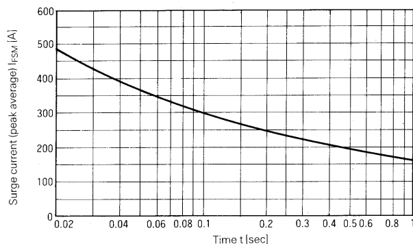
Surge Current
