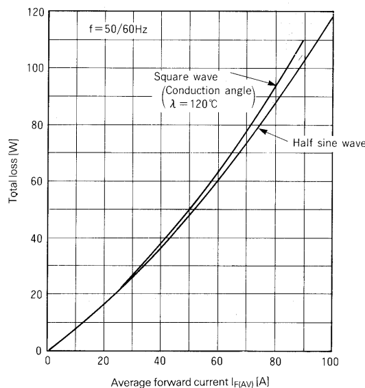
Power Loss — Forward Average Current
