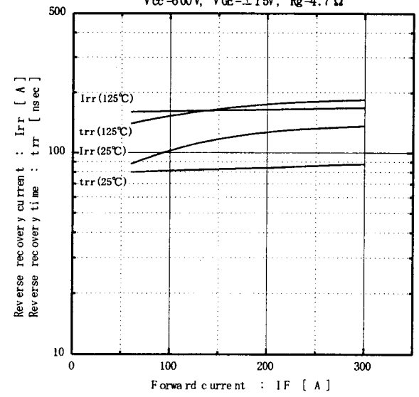
Reverse recovery characteristics (typ.) Vcc=600V, VGE=±15V, Rg=4.7Ω
