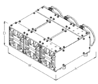
Figure 3 Weight 30 kg
