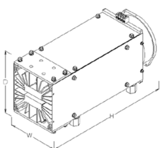
Figure 1 Weight 10 kg
