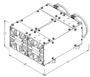
Figure 2 Weight 20 kg
