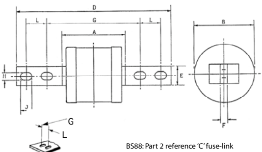
BS88: Part 2 reference 'C' fuse-link dimensions and tag variants
