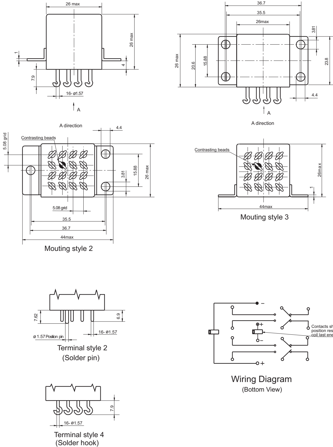
Outline Dimension
