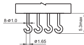
Terminal style 4 (Solder hook)
