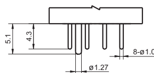
Terminal style 1 (Solder pin)
