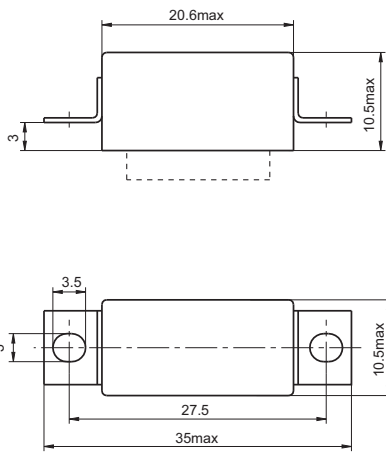
Mounting style 2
