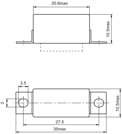
Mounting style 1
