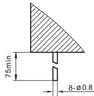
Terminal style 3 (Flexible terminal type)
