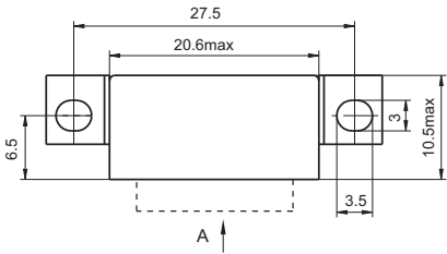
Mounting style 1
