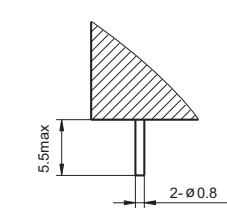
Coil Terminal Style 1 (Solder pin)
