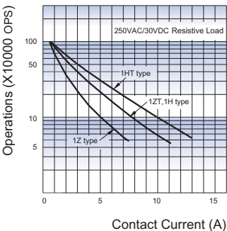
ENDURANCE CURVE
