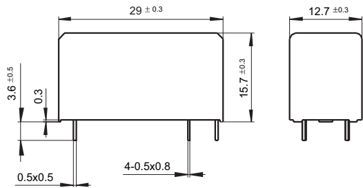
Outline Dimensions
